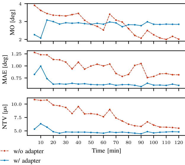
Fig. 16: Metrics evolution over the 2h duration of the experiment for the slow-aggressive PID controller. Each point represents the calculated value of the metric on identical 5min sequences of targets. Plots for all metrics and numerical values can be found in Figure C.1 and Table C.I, respectively.
