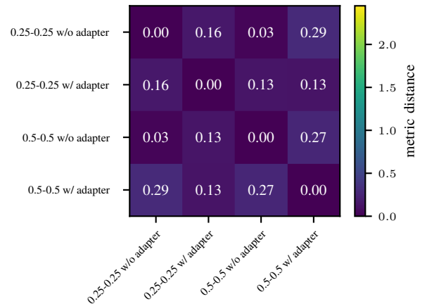
Fig. D.2: Distance in the metric space between the KOSs at the start of the 0.25–0.25mm and 0.5–0.5mm perforation experiment.
