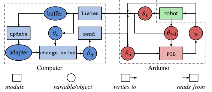
Fig. B.1: The interaction between the modules (rectangles) and shared variables (ovals) of the computer (blue) and Arduino (red).
