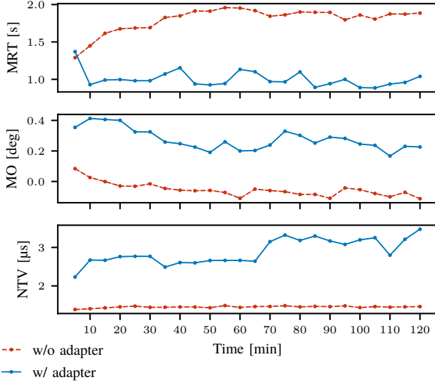
Fig. 17: Metrics evolution over the duration of the experiment for the under-tuned PID controller. Each point represents the calculated value of the metric on identical 5min sequences of targets. Plots for all metrics and numerical values can be found in Figure C.2 and Table C.II, respectively.
