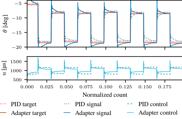
Fig. 26: Minute 1 of the pretrained adapter for the crawling gait experiment. Adaptations are immediately added to the target, resulting in worse behavior.
