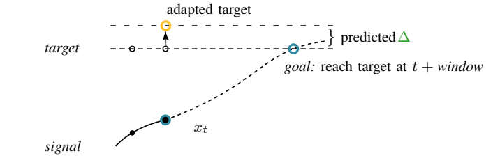
(a) By supplying the model with the controller’s target position and current state x_t , it yields a \Delta that can be added to the current target, which will supposedly result in the controller reaching the target within the specified window.
