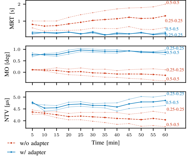
Fig. 19: Metrics evolution over the 1h duration of the experiment for KOSs in a lower state of degradation (0.25–0.25mm and 0.5–0.5mm perforations, see annotations), with their average overlayed. Each point represents the calculated value of the metric on identical 5min sequences of targets. Plots for all metrics and numerical values can be found in Figure C.3 and Table C.III, respectively.
