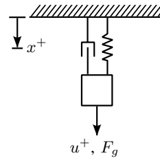
Fig. 6: Setup of the mass-spring-damper system in the illustrative problem with positive directions indicated.
